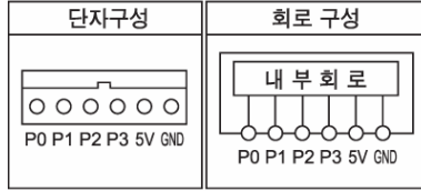
▶ [CN16] KEYPAD
